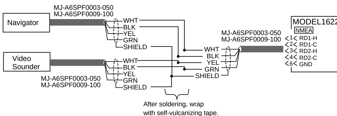
Figure 15 Connection of video sounder and navigator cables
