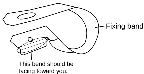
Figure 9 Fixing band
