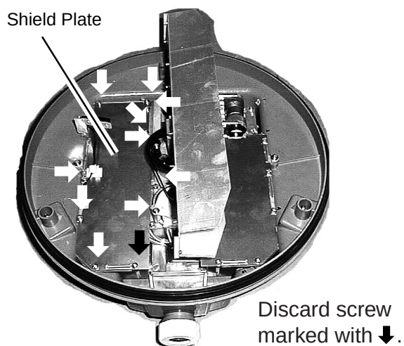
Figure 6 Antenna unit, inside view
