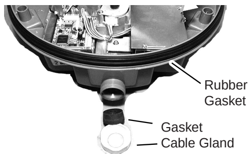
Figure 7 Antenna unit, inside view
